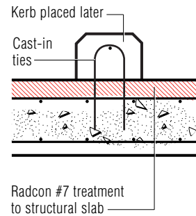
DETAIL PM1 KERB
